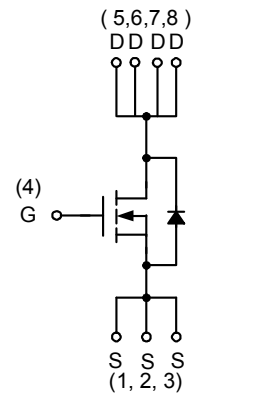
N-Channel MOSFET
